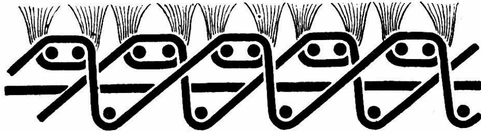
FIG. 24 TAPESTRY VELVET. 3-SHOT
