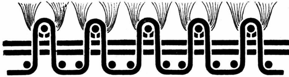
FIG. 26 TAPESTRY VELVET. 2 SHOTS IN THE GROUND
