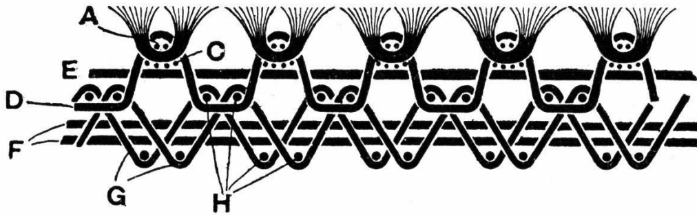
FIG. 14 SECTION OF CHENILLE AXMINSTER
